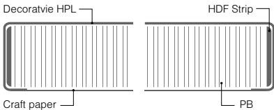
Profile U-U R = 3.3 mm
